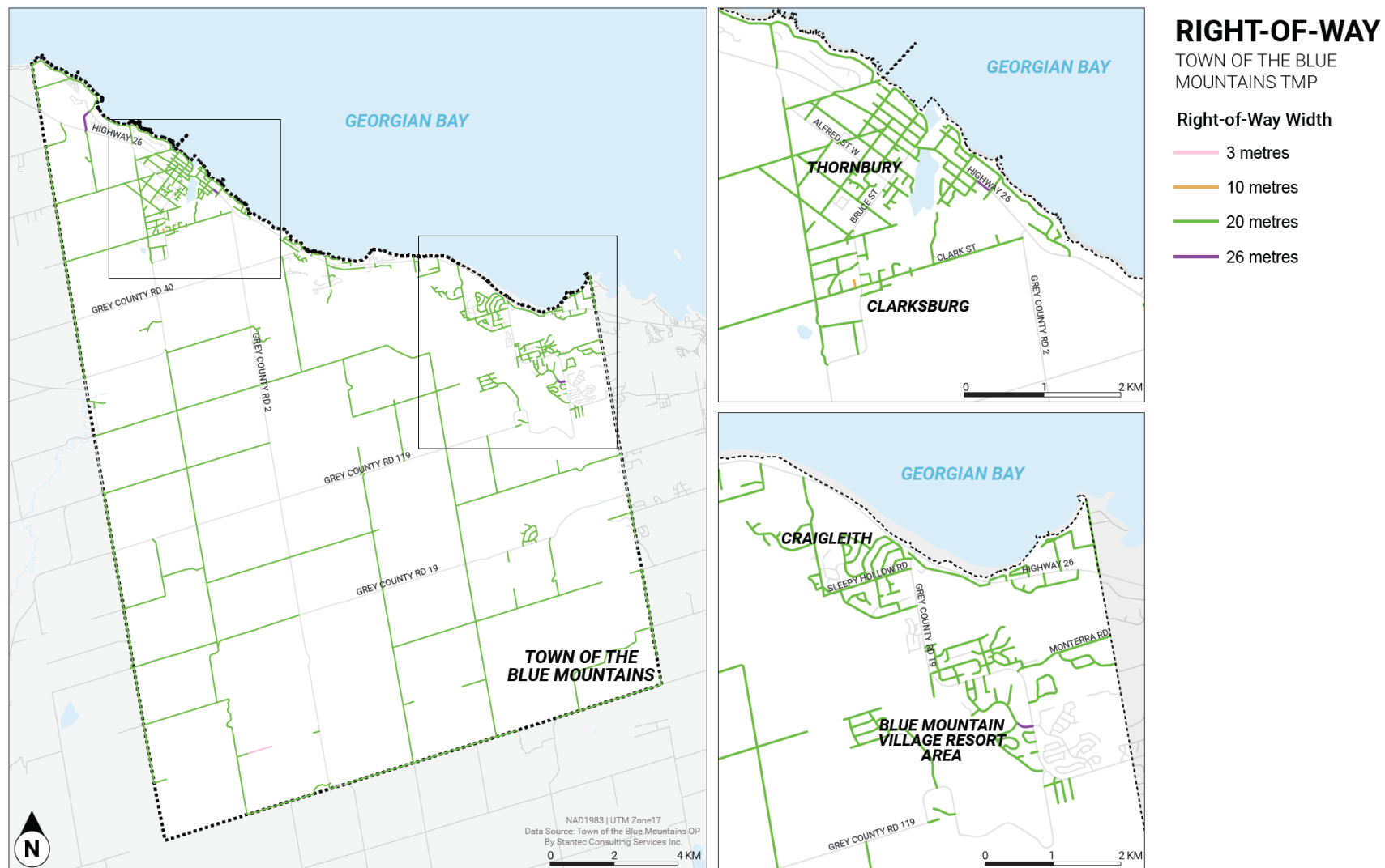
Figure 4-9: Existing Right-of-Way Widths in TBM
