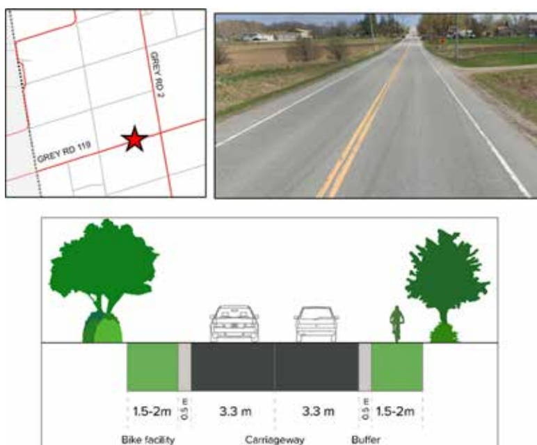
Figure 8-8: Potential Cross-Section Treatment for Grey Road 119
