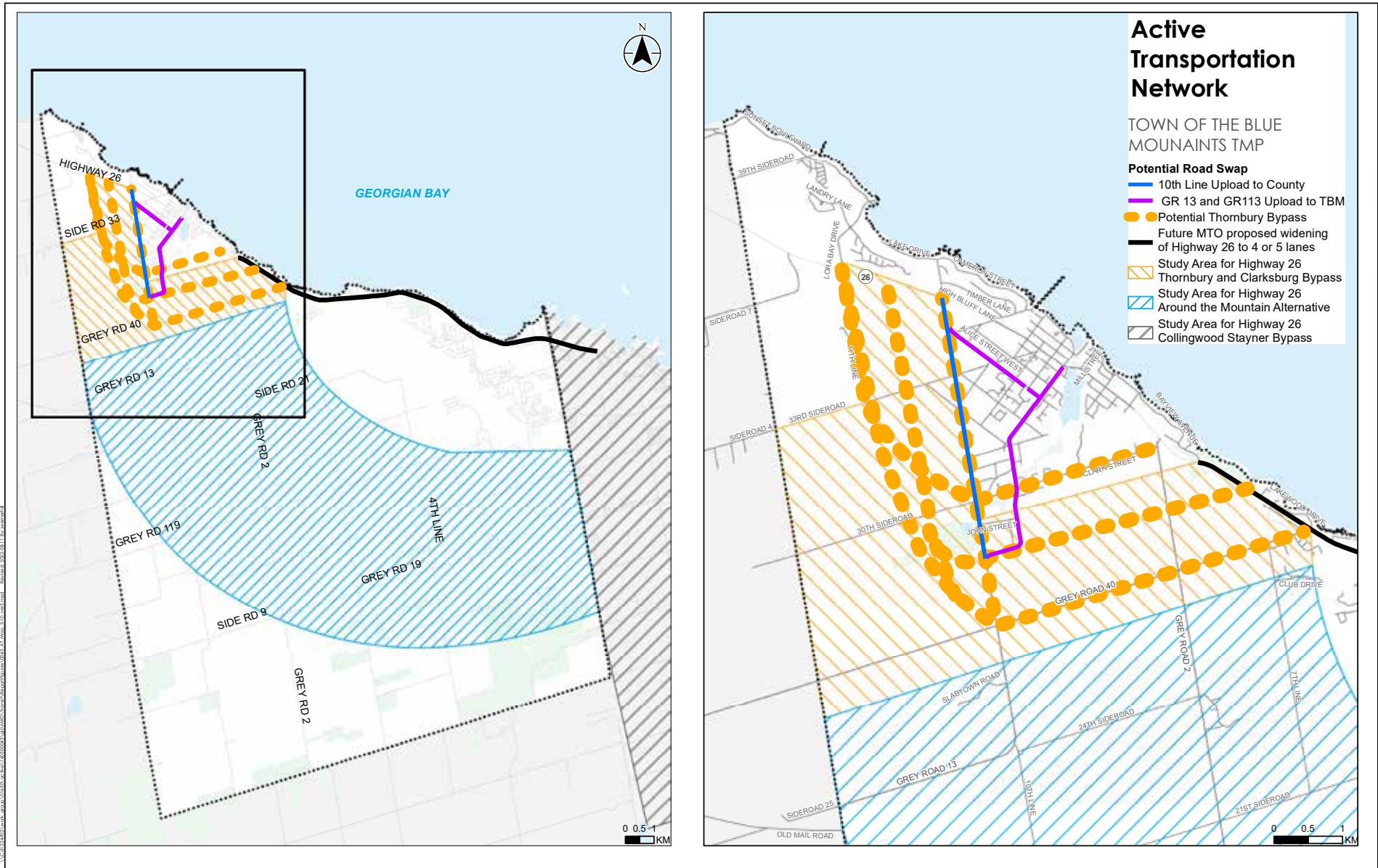
Figure 8-2: Highway 26 Widening & Bypass Study Areas & Potential Alignments
