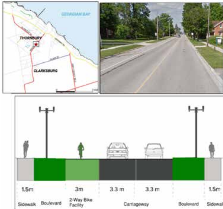
Figure 8-9: Potential Cross-Section Treatment for Bruce Street
