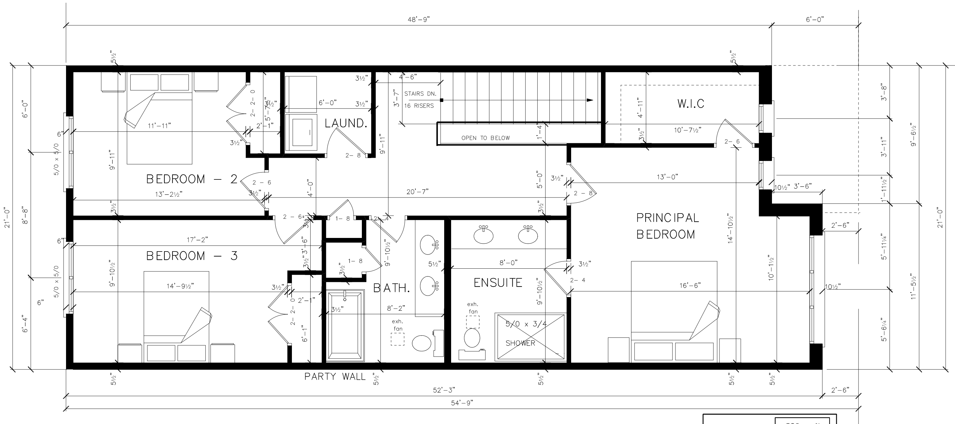
UPPER FLOOR PLAN ( INSIDE UNIT ) - B
