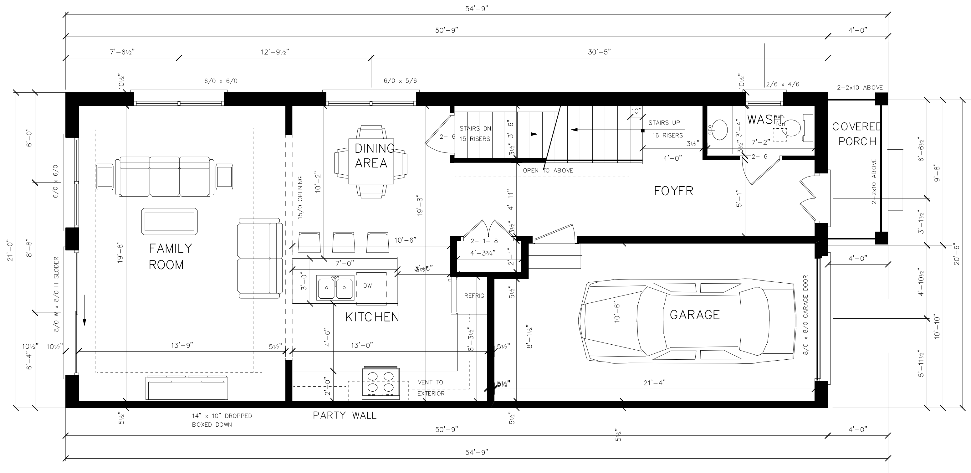
MAIN FLOOR PLAN ( RIGHT ) CORNER
