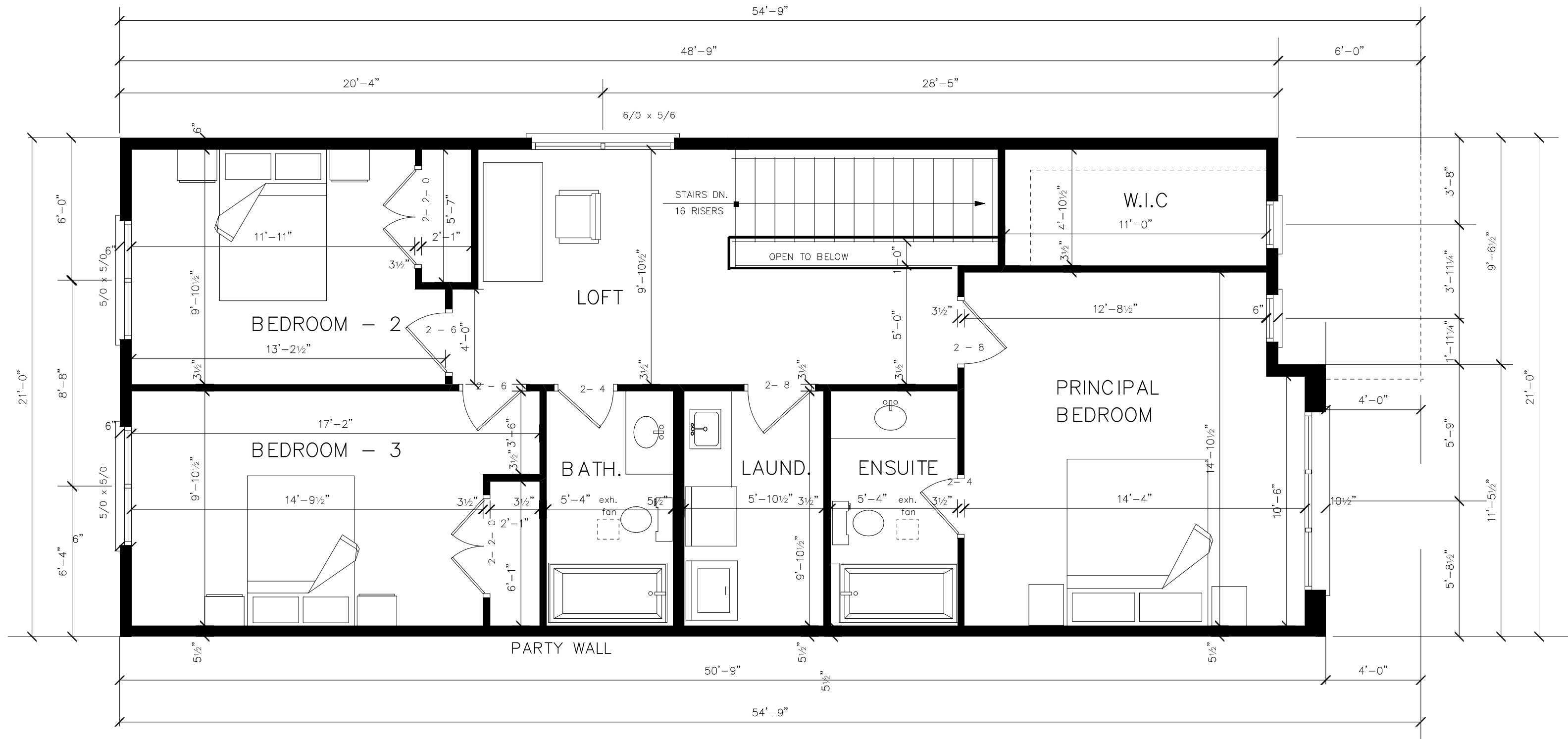
UPPER FLOOR PLAN ( RIGHT ) CORNER
