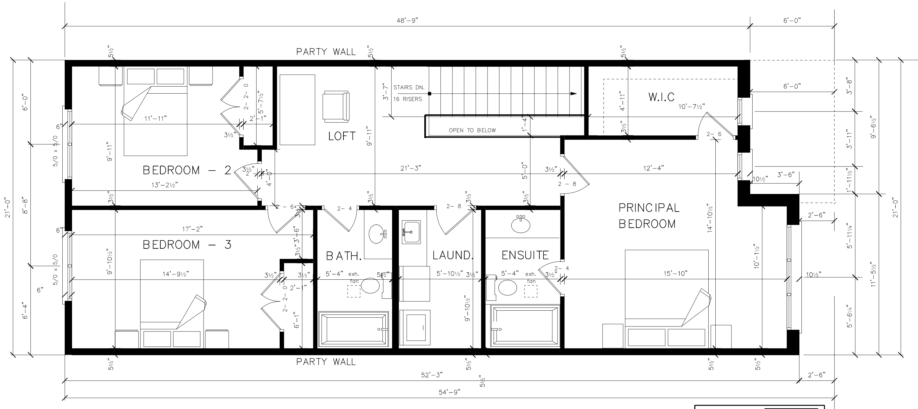
UPPER FLOOR PLAN ( INSIDE UNIT ) - A
