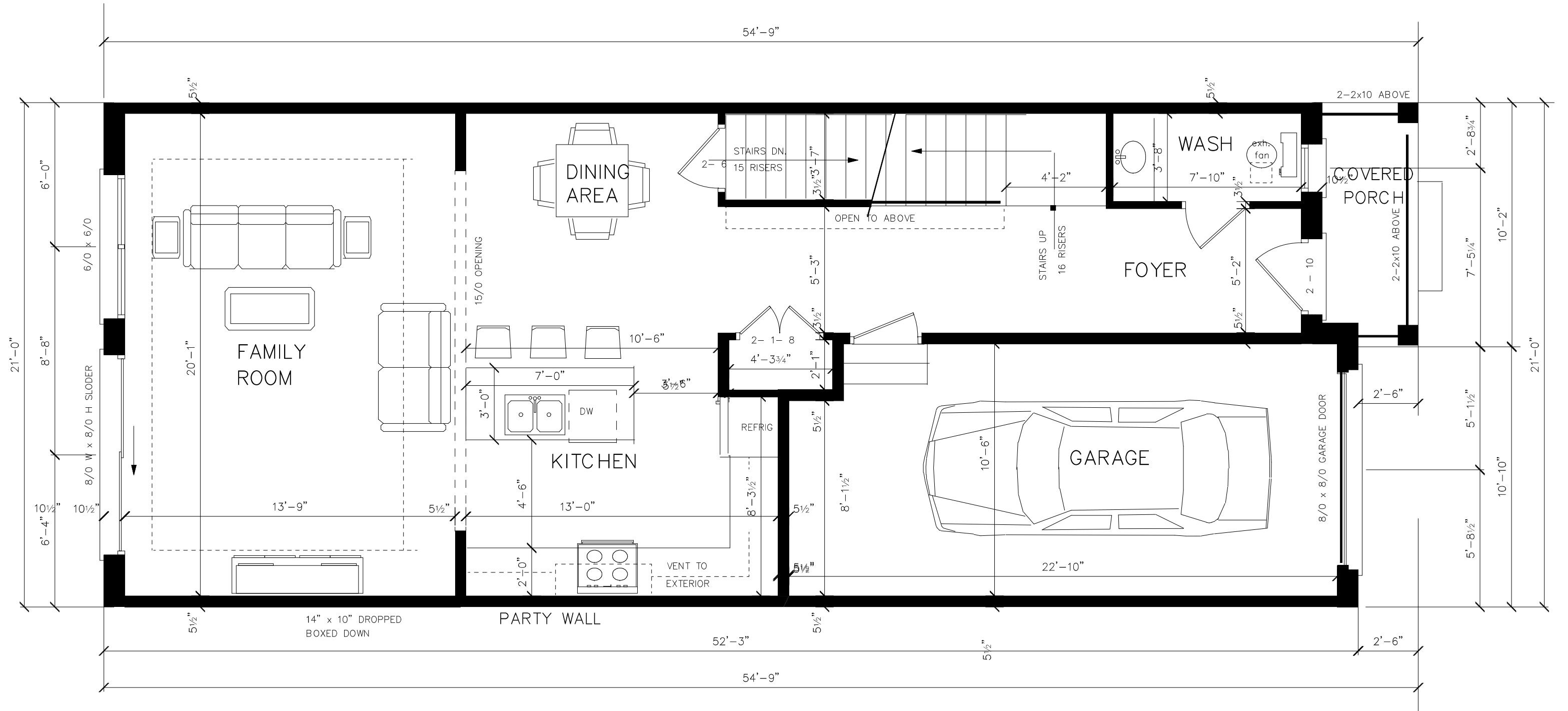
MAIN FLOOR PLAN ( INSIDE UNIT )
