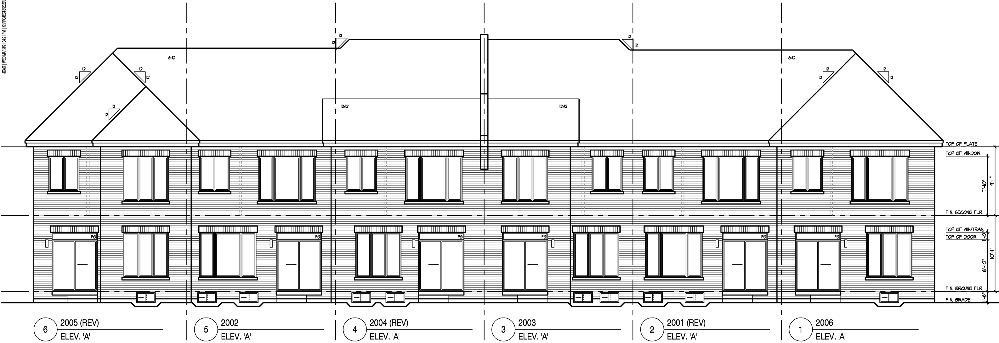
REAR ELEVATION 'A' BLOCK OF 6
