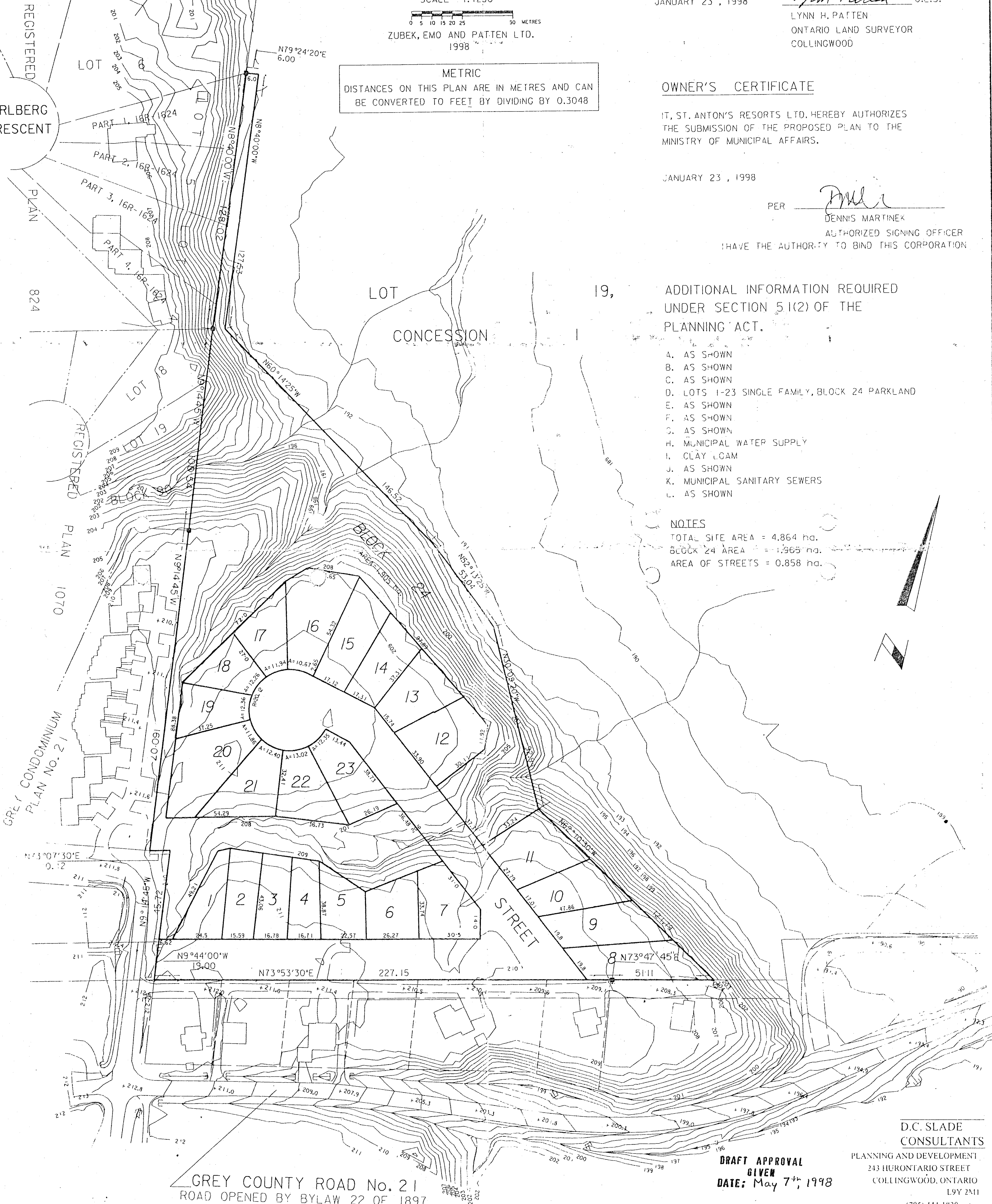
KEY PLAN
