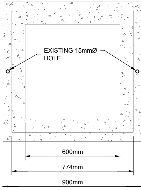
EXISTING PRECAST CONCRETE DETAIL, TOP VIEW
