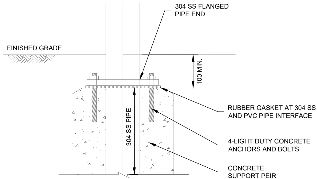
VENT PIPE CONNECTION DETAIL
