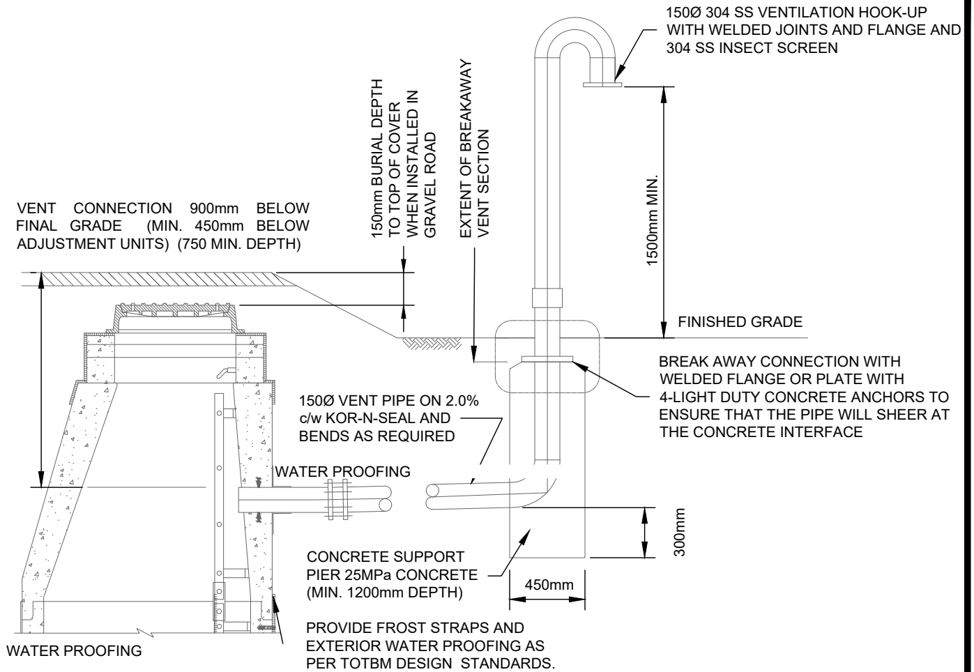
MAINTENANCE HOLE VENTING DETAIL
