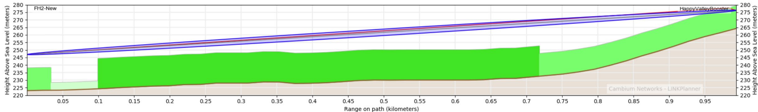
Profile: 0.994 kilometers, Non Line-of-Sight
